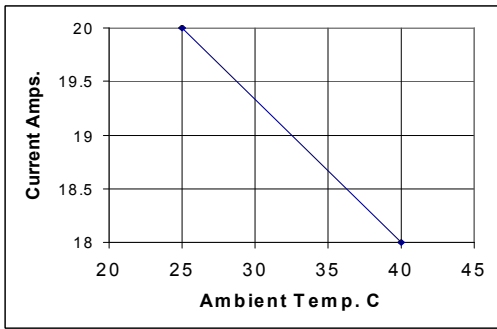
Derating Curve show is for 277V 20A models
