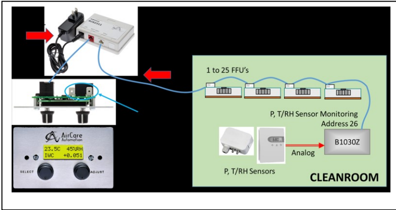
ACM1005 – Wall Mount
